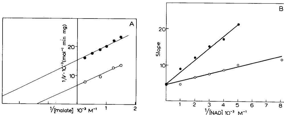
Fig. 6. Secondary plots for the effect of thenoyltrifluoroacetone with respect to malate concentration. (A) The effect of thenoyltrifluoroacetone on intercept of primary plots. \circ , no inhibitor; \bullet , 15 \mu\text{M} thenoyltrifluoroacetone; K_i = 11 \mu\text{M} . (B) The effect of thenoyltrifluoroacetone on the slopes of primary plots. Ordinate d(v)^{-1}/d[\text{malate}]^{-1} ; abscissa [\text{NAD}]^{-1} . \circ , no inhibitor; \bullet , 15 \mu\text{M} thenoyltrifluoroacetone; K_i = 6.4 \mu\text{M} .
