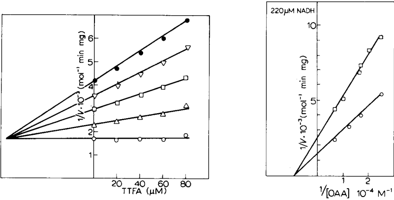
Fig. 2. Dixon plot for inhibition of NADH oxidation by malate dehydrogenase by thenoyltrifluoroacetone at constant oxaloacetate concentrations (197 \mu\text{M} ). NADH: \bullet , 25 \mu\text{M} ; \Delta , 33 \mu\text{M} ; \square , 50 \mu\text{M} ; \triangle , 100 \mu\text{M} ; \circ , \infty .
