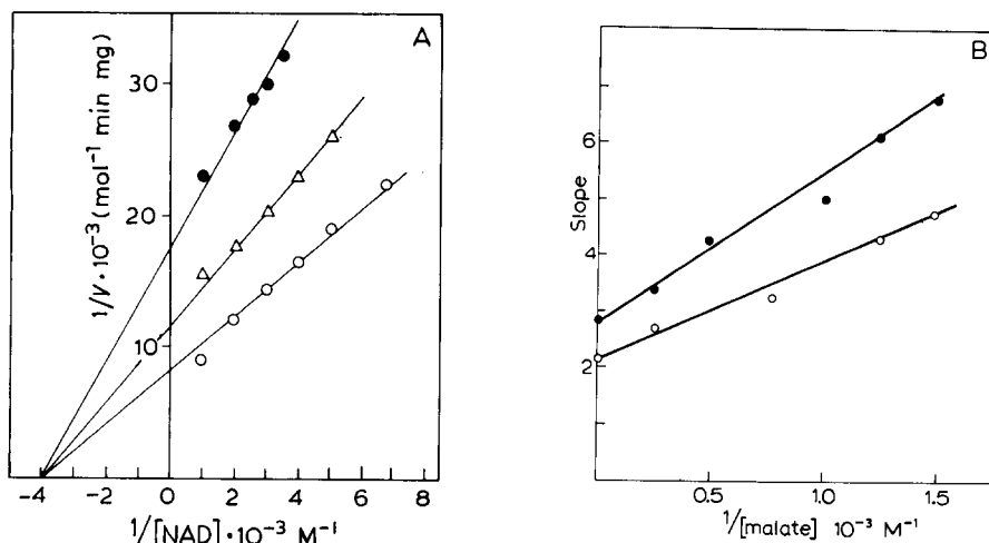
Fig. 5. Secondary plots for the inhibition of by thenoyltrifluoroacetone of NAD reduction by malate dehydrogenase. (A) The effect of thenoyltrifluoroacetone on intercepts of primary plots. \circ , no inhibitor; \Delta , 15 \mu\text{M} thenoyltrifluoroacetone; \bullet , 30 \mu\text{M} thenoyltrifluoroacetone; K_i = 20\text{--}25 \mu\text{M} . (B) The effects of thenoyltrifluoroacetone on the slope of primary plots. Ordinate d(v)^{-1}/d[\text{NAD}]^{-1} ; abscissa [\text{malate}]^{-1} . \circ , no inhibitor; \bullet , 15 \mu\text{M} thenoyltrifluoroacetone.
